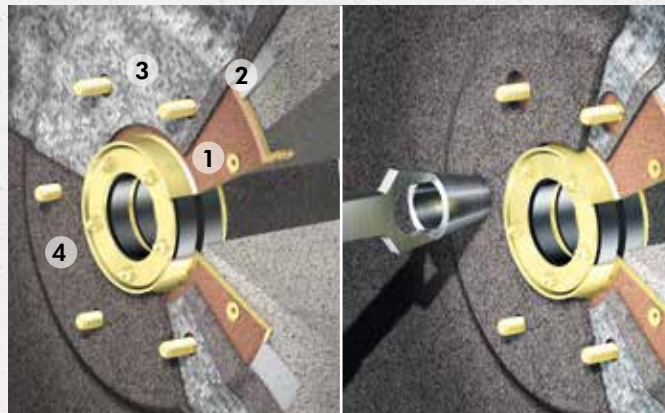
Layers from bottom to top: sanding (1), thick coating (2), fleece insert (3), thick coating (4)
