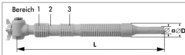
Abb. 6: Type HSP-SKE- ...
